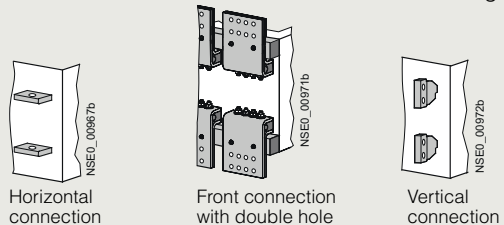
Main circuit connections
